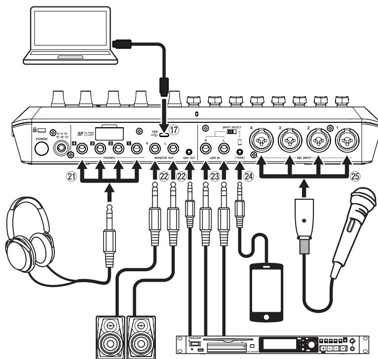
Panel trasero
