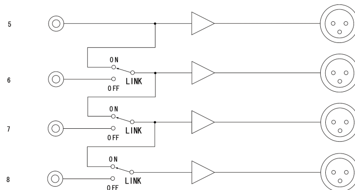
(UNBALANCE→BALANCE)
