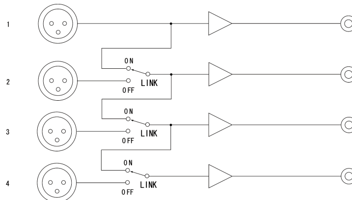
(BALANCE→UNBALANCE)
